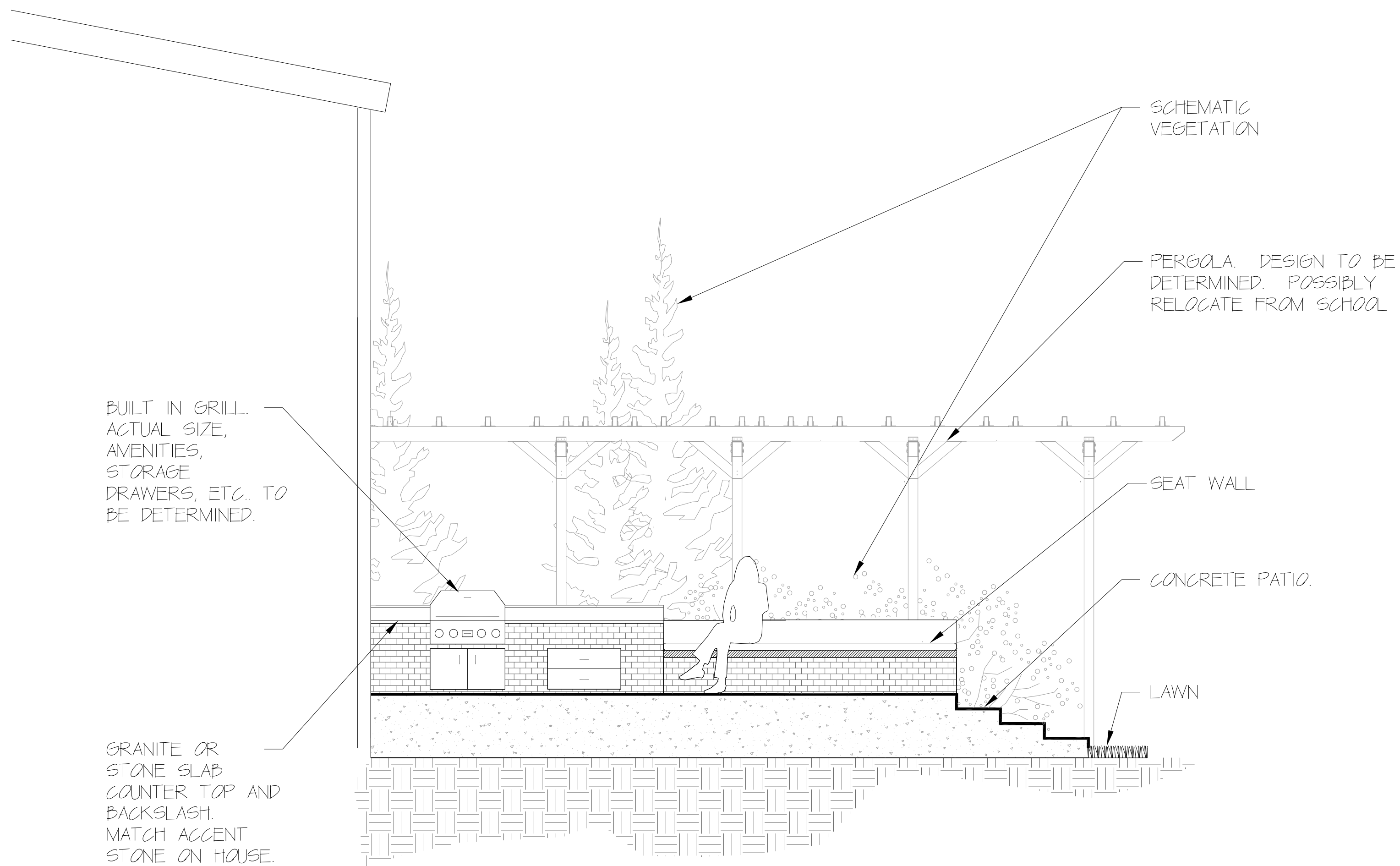
Ⓐ OUTDOOR GRILL SCHEMATIC SCALE: 1" = 3'-0" WHEN PRINTED @ 24"X36"
